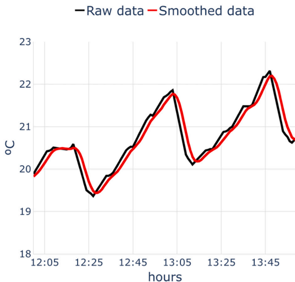
Fig. 12. Smoothing process applied to several hours of temperature data acquired with the mobile device.
