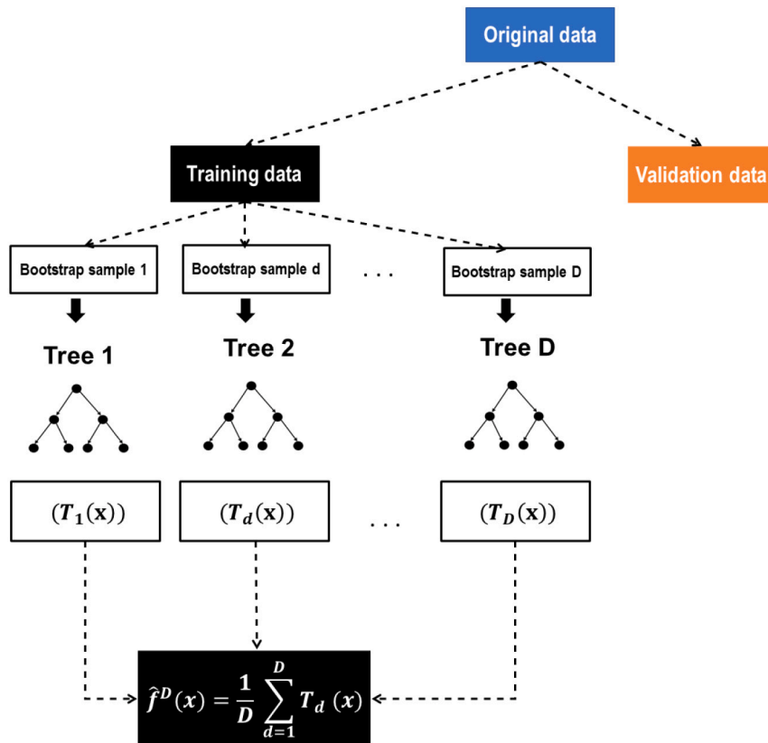
Fig. 8. Summary of the training process for the Random Forest algorithm. The way of obtaining the final output as a combination of the outputs of the individual trees ( T_d(x) ) is also presented.
