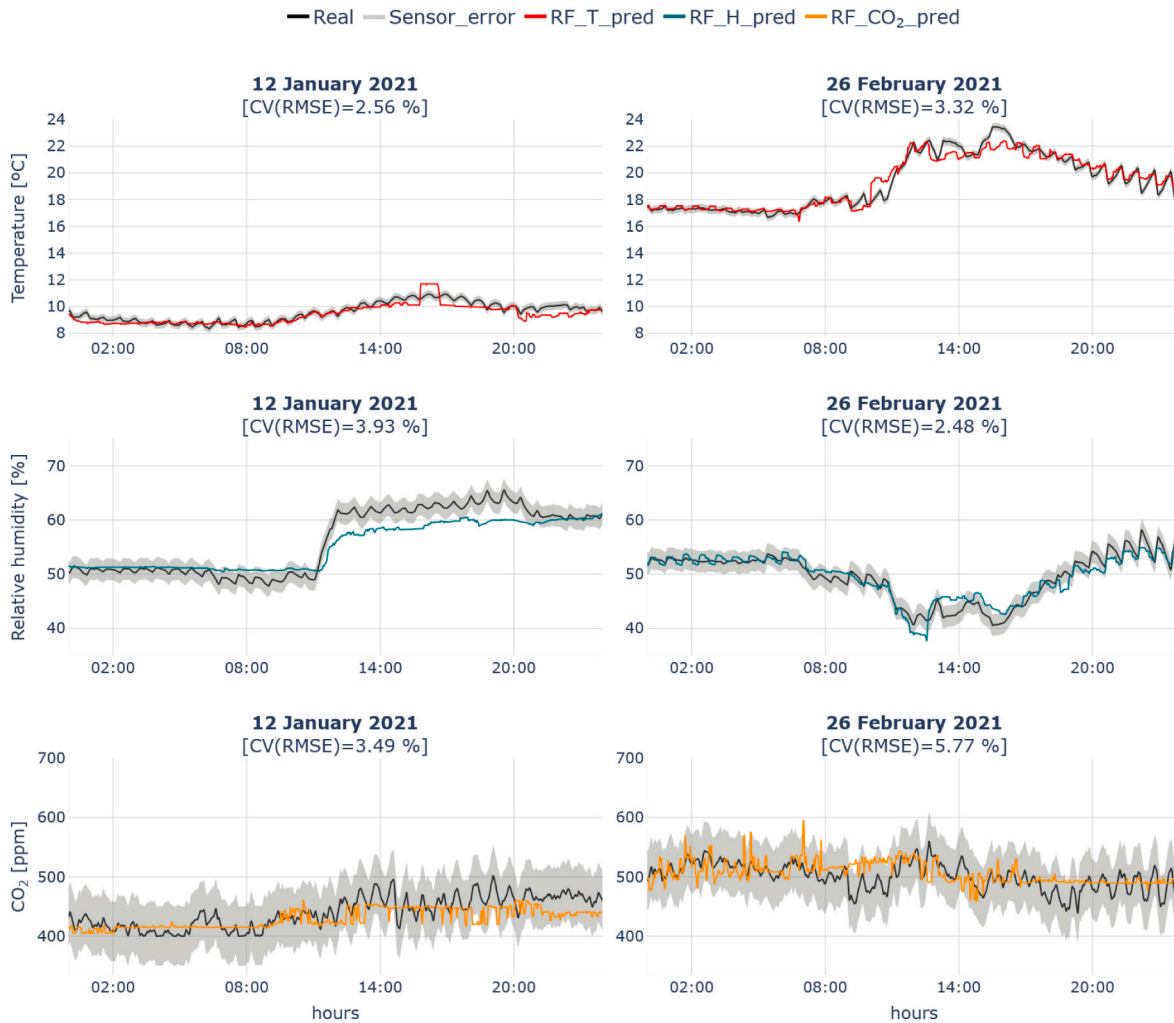
Fig. 14. Results of the interpolations made with the RF model in specific days and, thus, in positions known by the mobile device, together with the errors obtained. Indoor temperatures are presented in the first row, relative humidity in the second and CO 2 concentration in the third.
