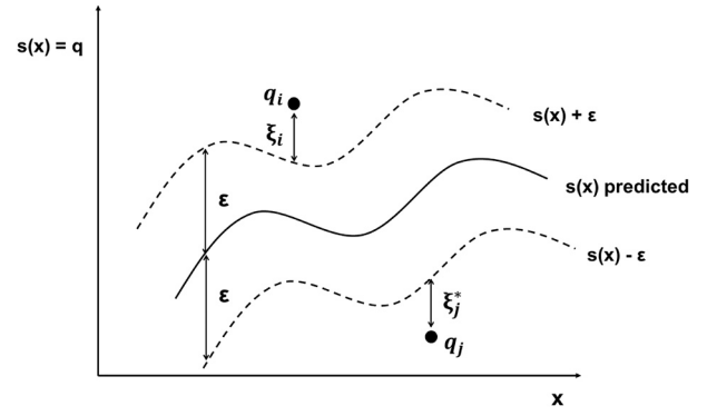
Fig. 9. SVR parameters considered in the training process.
