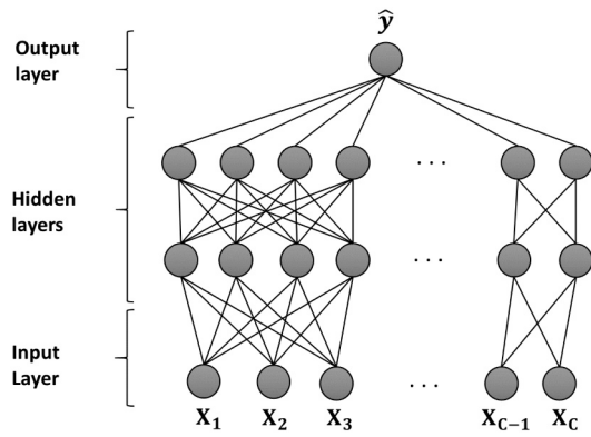
Fig. 7. MLP architecture with an input layer, several hidden layers and an univariate output layer.
