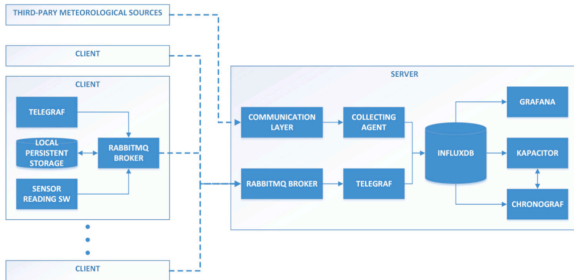
Fig. 3. High-level block diagram of the software platform, exposing the underlying client-server architecture.
