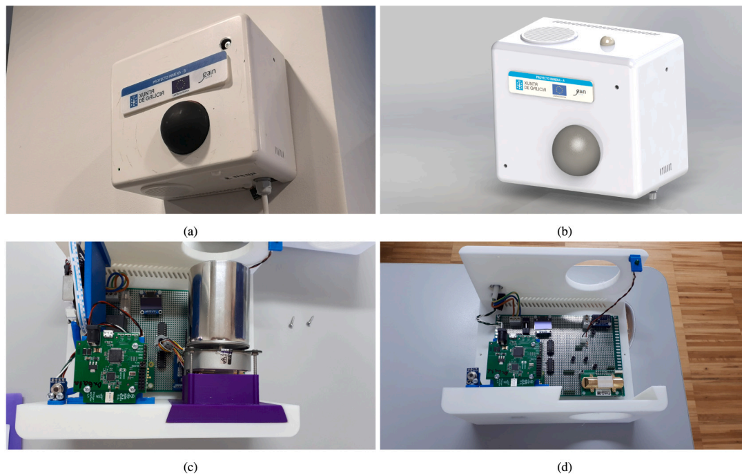
Fig. 1. Wall-mounted devices: (a) installed device; (b) CAD model; (c) internal design for WMA and (d) for WMB, with WMC being almost identical to WMC.
