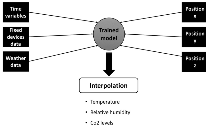
Fig. 13. Summary of the interpolation process after train the machine learning method. Black boxes represent the inputs and the list of variables the outputs from the interpolation process.
