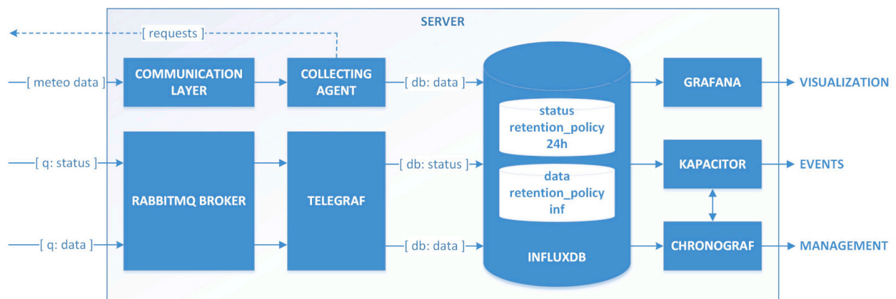
Fig. 5. High-level block diagram of the server node.
