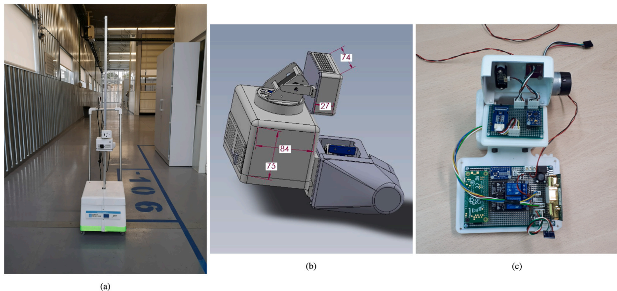
Fig. 2. Mobile device: (a) assembled device; (b) CAD model of the header, with distances in mm; (c) internal design with the sensors.
