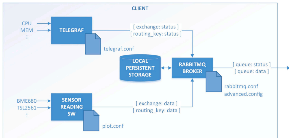
Fig. 4. High-level block diagram of the client node.
