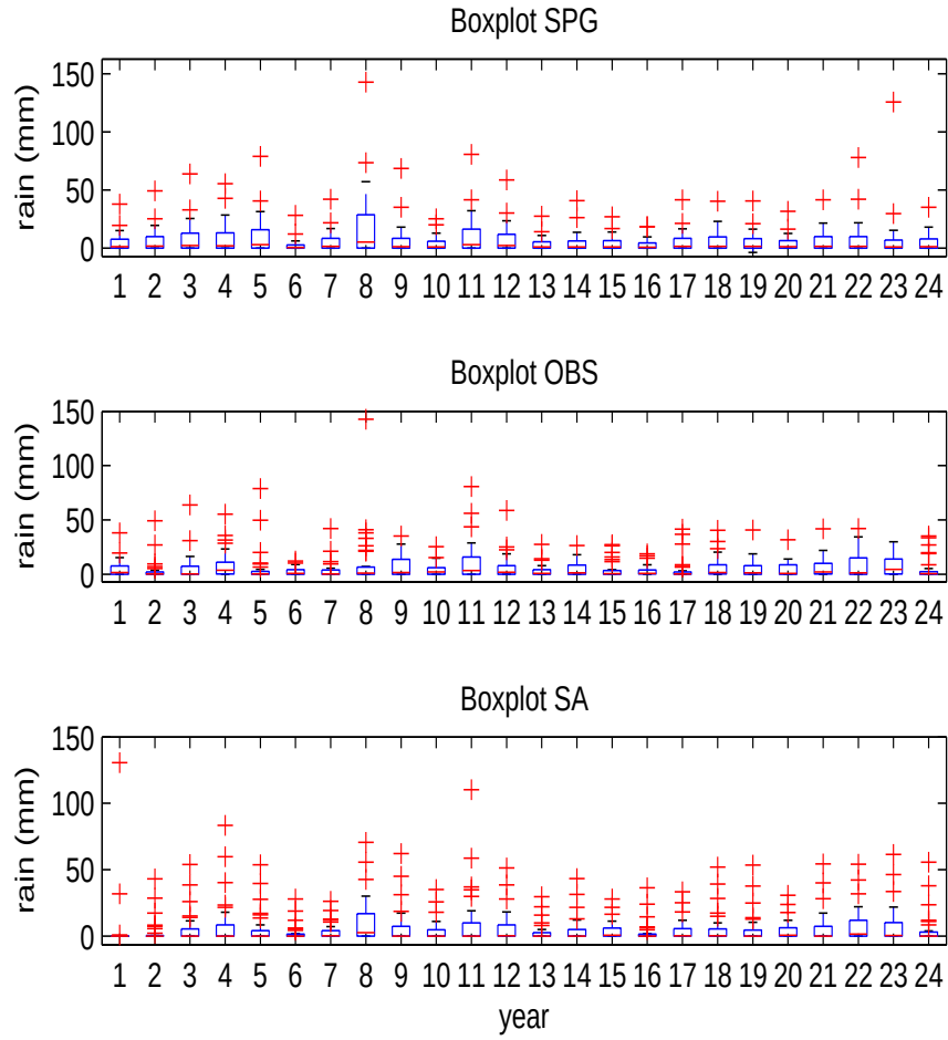
Fig. 4: Boxplots for the EDR series obtained with SA and SPG methods vs. the observed disaggregated sequences for the month of August
