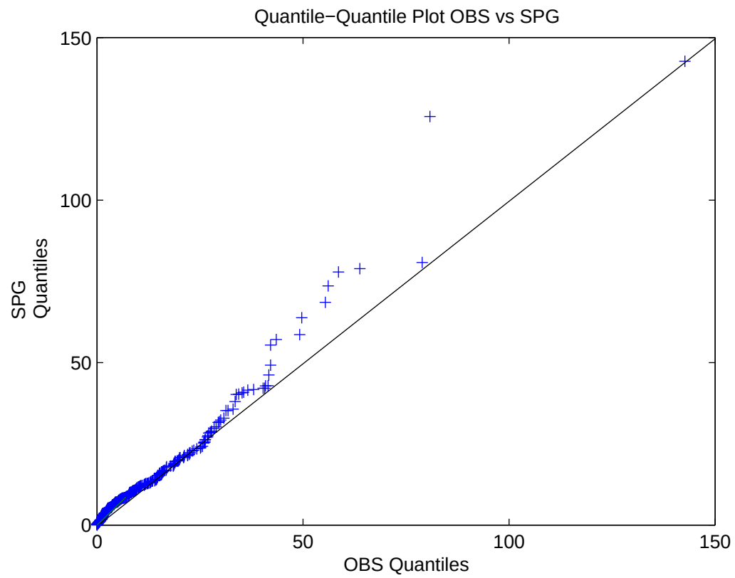
Fig. 2: Quantile-Quantile plot of the EDR series obtained with the SPG method
