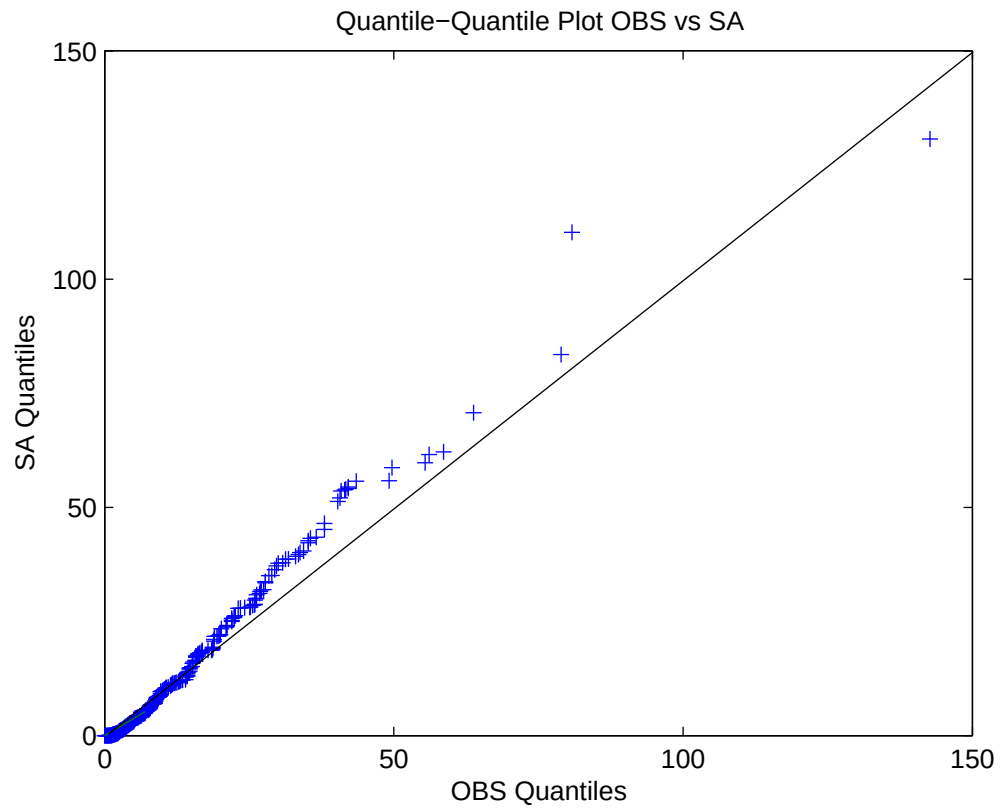
Fig. 1: Quantile-Quantile plot of the EDR series obtained with the SA method
